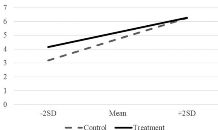
Figure 3. Effect of ST Math on Self-Beliefs Moderated by Prior Achievement. Regression-adjusted unstandardized coefficients graphed at three points separately for treatment and control: the mean of pooled achievement, two standard deviations below the mean, and two standard deviations above.
